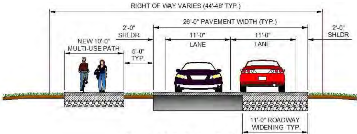
Option 1A Multi-Use Path On West Side of Carr Road
