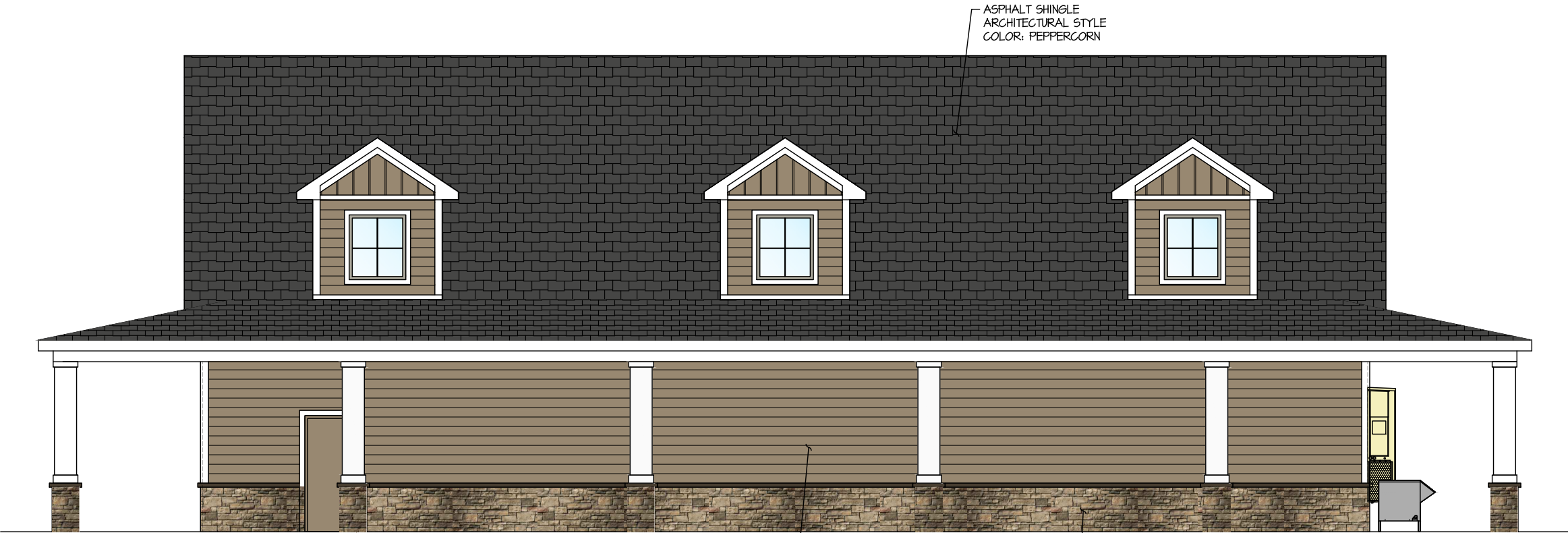
NORTH BUILDING ELEVATION
