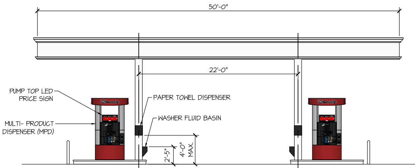
GAS CANOPY WEST ELEVATION
